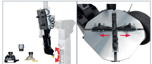
incl. quick-action chuck and pneumatic mounting finger
