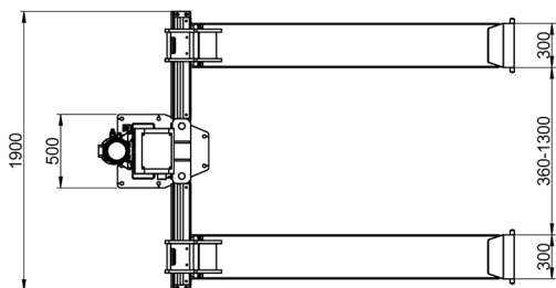
360mm with optional accessories (wheel clamps)
