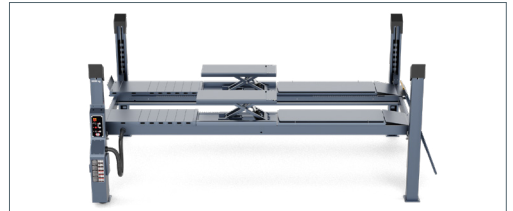
Wheel-free jack (load capacity 3.5 t) with wheel alignment kit
