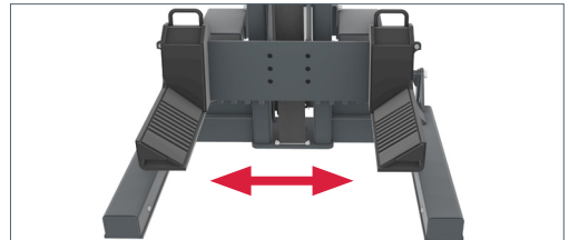
Adjustable pickup 166 mm to 550 mm
