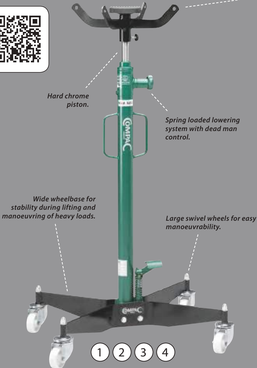
Reversible transmission adaptor with saddle and rubber pad.
