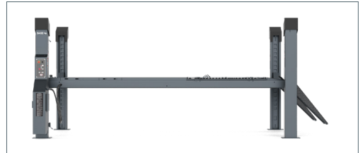
ATH Four Lift 46AP / 64AP Level guide rail with axis measurement kit
